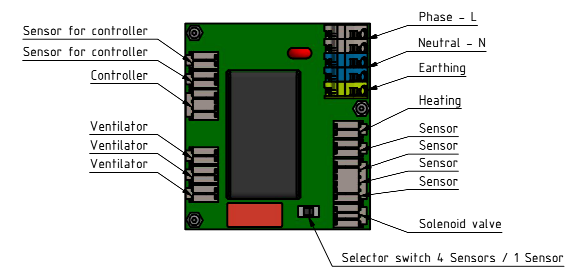
Circuit board ( 1 : 2 )
